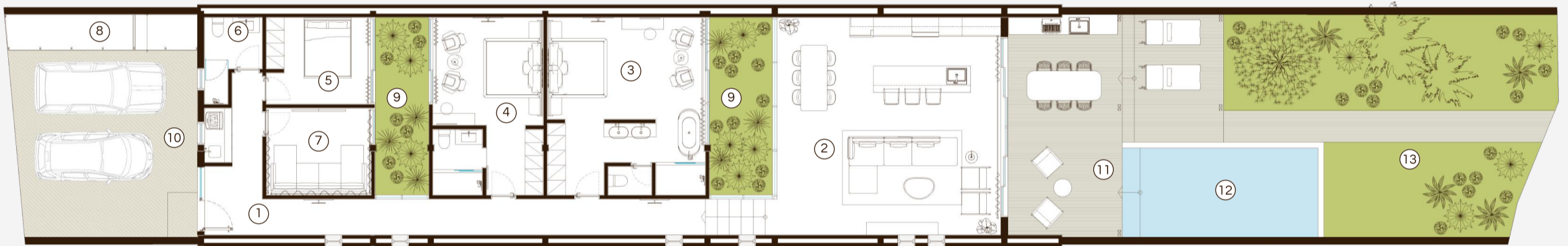
3 BEDROOM CORNER VILLA LAYOUT
